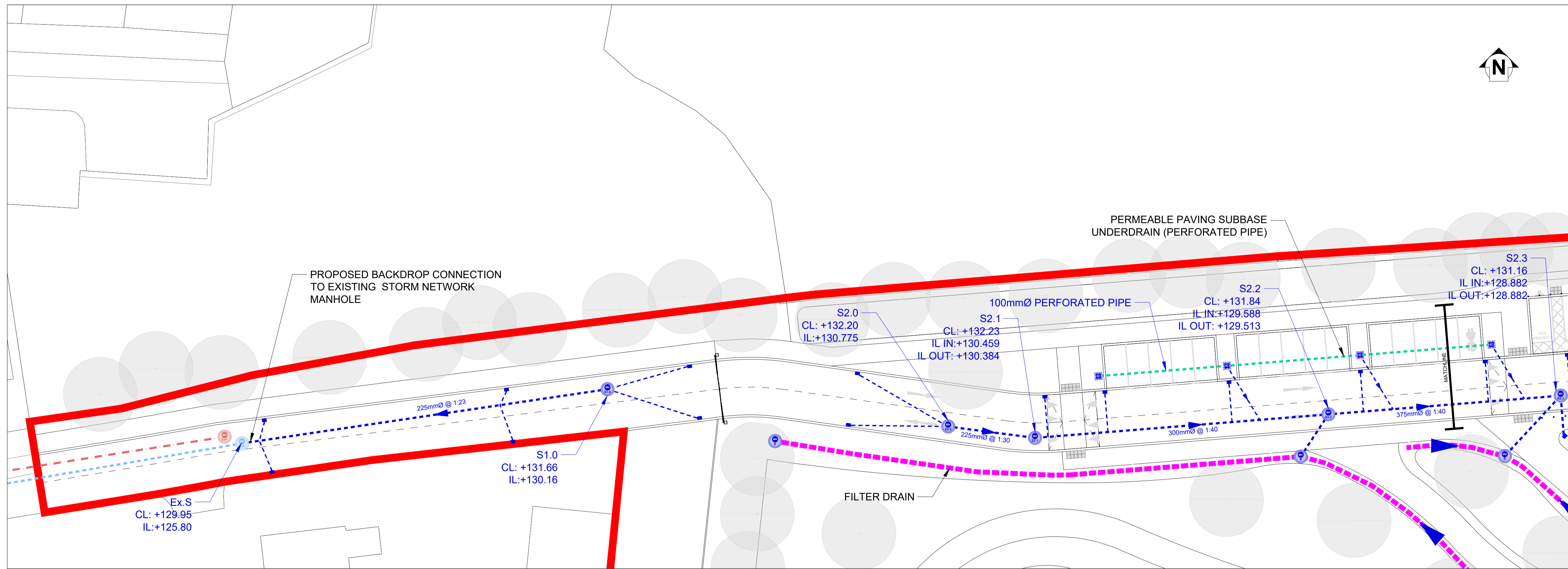
PLAN LAYOUT (WEST)
