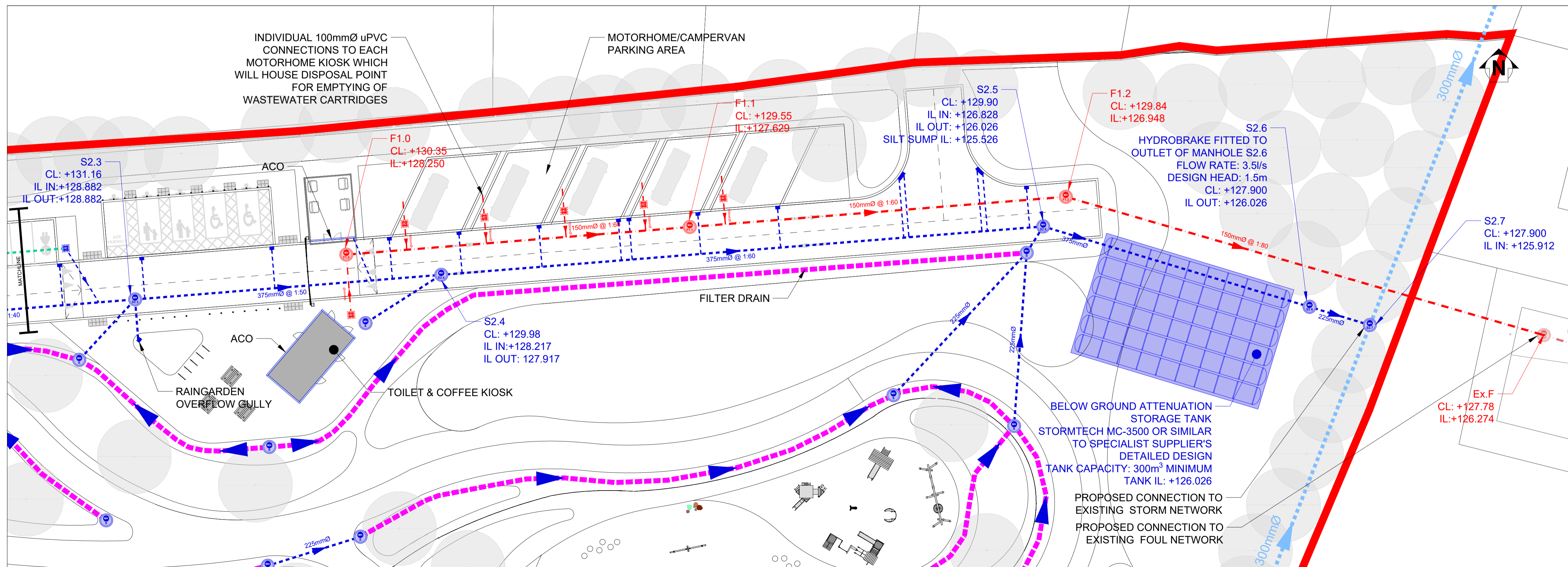
PLAN LAYOUT (EAST)
