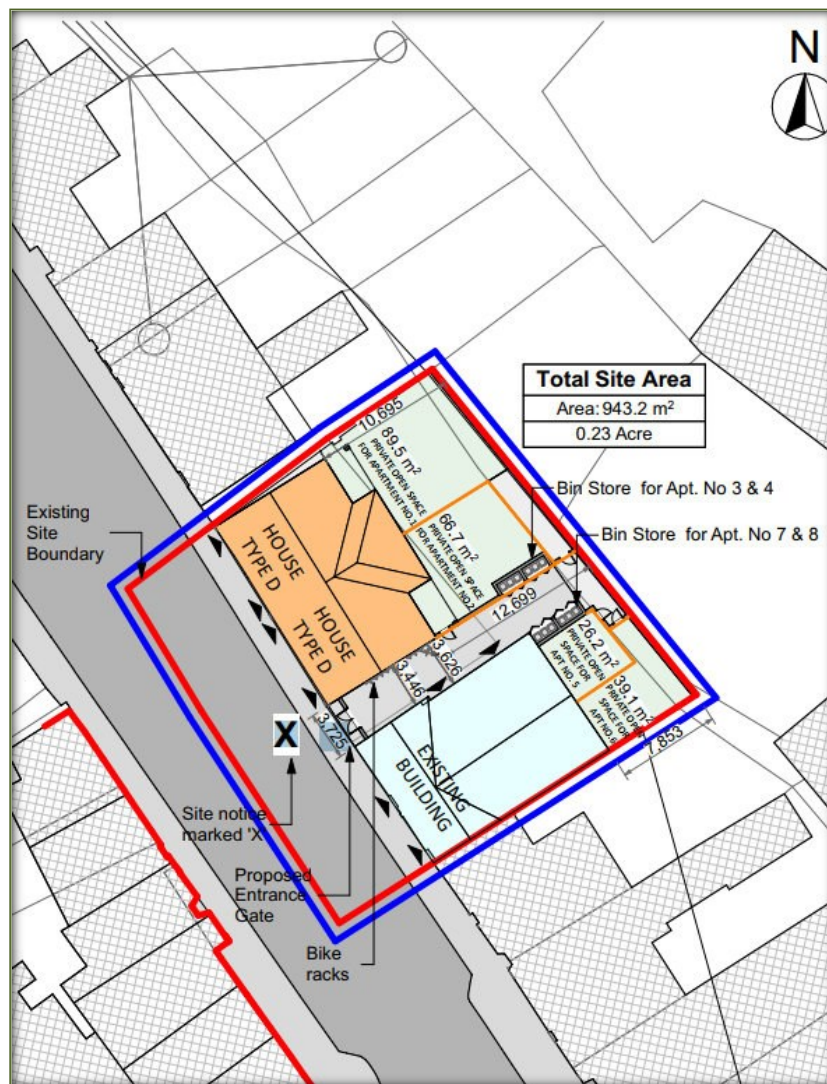
Figure 1a –Site Plan (as prepared by WGG Architects)
